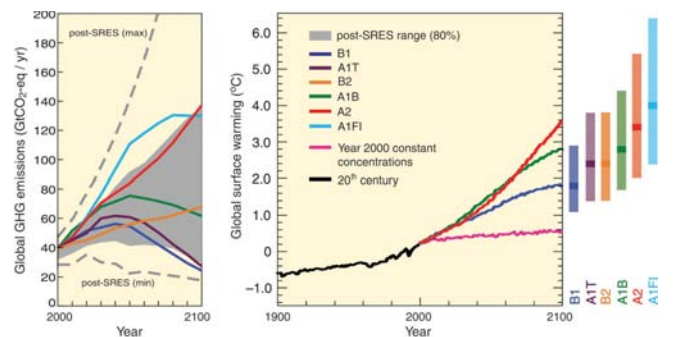
In this graphic from the Intergovernmental Panel on Climate Change (IPCC) Assessment Report 4 (Figure SPM.5), colored lines represent projections from six different emission scenarios developed in the IPCC’s 2000 Special Report on Emission Scenarios (SRES). Each scenario represents emissions resulting from a set of assumptions about world economic and population growth rates, and the adoption of varying degrees of resource-efficient technologies. The panel on the left shows greenhouse gas emissions in the absence of climate policies: six SRES scenarios and the 80th percentile range of recent scenarios published since the SRES (gray shaded area). The panel on the right shows the surface warming projections for the SRES scenarios. The pink line is not a scenario, but represents simulations where atmospheric concentrations of greenhouse gases are held constant at year 2000 values. The bars at the right indicate the likely range of the SRES scenarios for 2090–2099. All temperatures are relative to the period 1980–1999. Credit: Intergovernmental Panel on Climate Change (IPCC) Assessment Report 4 (Figure SPM.5), www.ipcc.ch/index.htm
